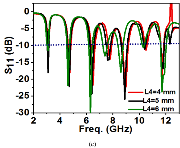
Fig. 4. Parametric study of (a) L_3 , (b) L_5 and (c) L_4
