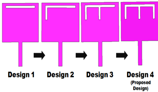
Fig. 2. Evolution steps of the proposed antenna structure.
