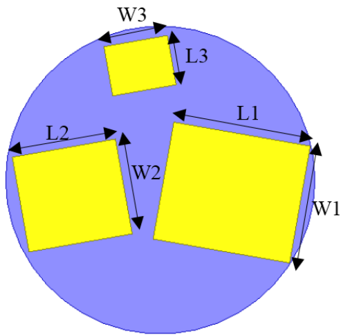
Fig. 5. Three shapes patch module.
