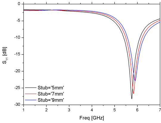
Fig. 13. Return loss values vs frequency by varying Stub at position 2.
