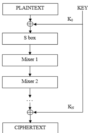
Figure 1. Qamal encryption algorithm block diagram
