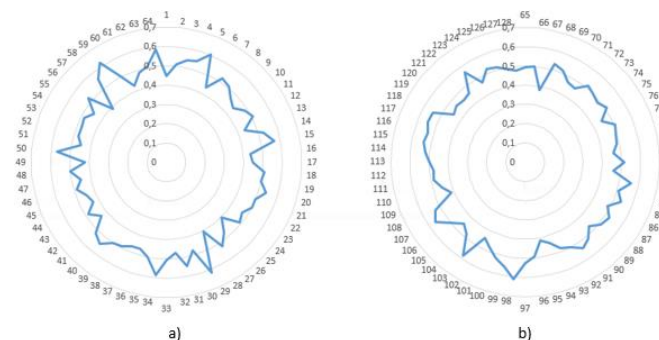
Figure 4. Analysis of the avalanche effect for a key in the full-round algorithm Diagrams of k_i values for index i : a) from 1 to 64, b) from 65 to 128
