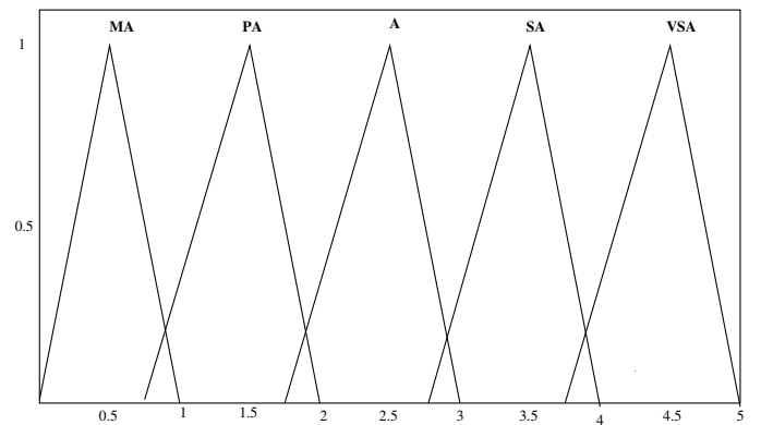
Fig. 5. Membership function plot for CH selection
