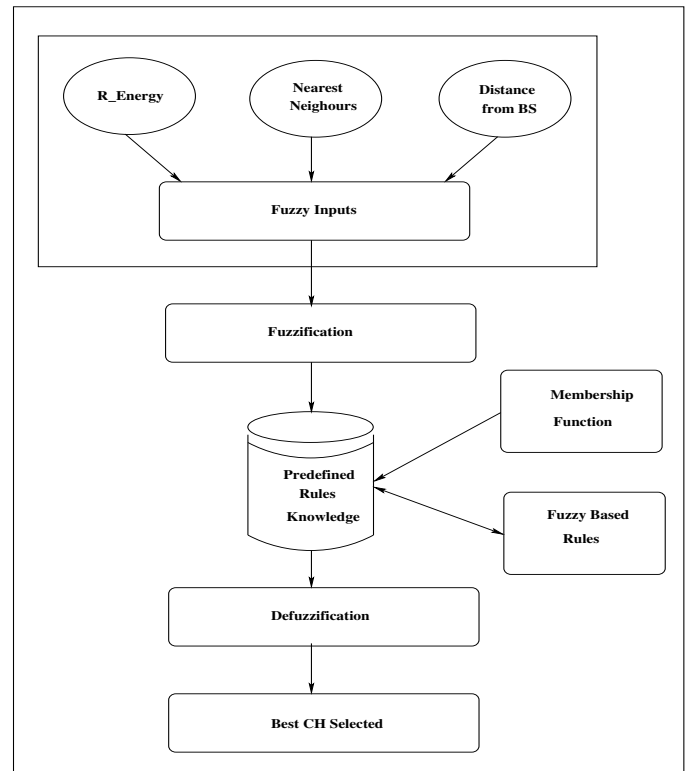
Fig. 4. Fuzzy Inference System for Cluster Head Selection
