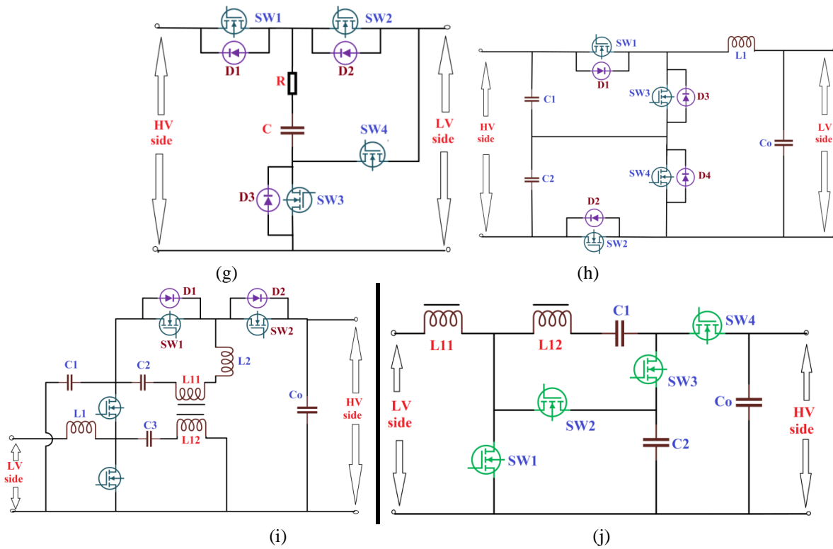
Fig. 7. Bidirectional Non-Isolated DC-DC converter (a) BNIRC (b), (i) and (j) BNICIC (c) and (d) BNISSC (e) BNIC (f) BNICC (g) BNISCC (h) BNISSC
