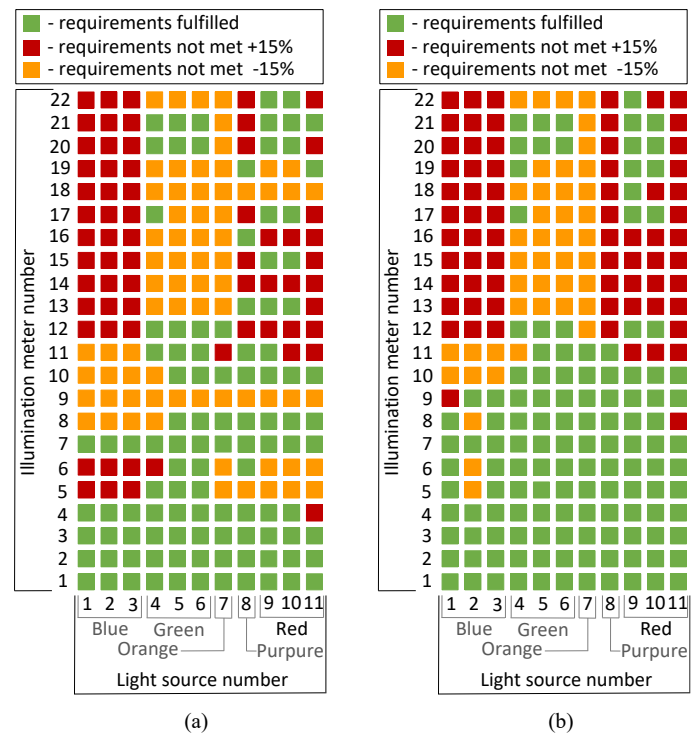
Fig. 11. Graphic illustration of the evaluation of photometers in terms of illuminance values resulting from (a) laboratory measurements, (b) calculations
